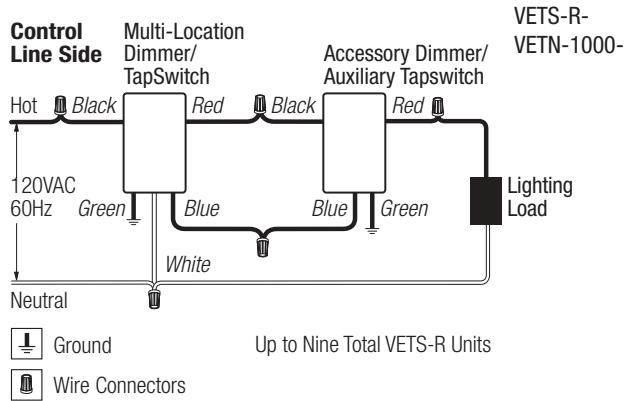
Wiring Diagram 4 Multi-Location Wiring
