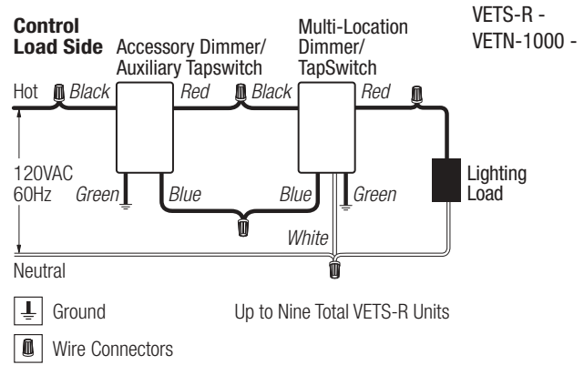
Wiring Diagram 7 Multi-Location Wiring
